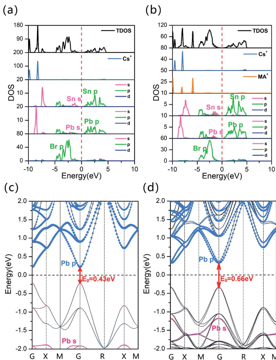
Fig. 5 TDOS and PDOS of (a) CsSn 0.5 Pb 0.5 Br 3 and (b) MA 0.5 Cs 0.5 Sn 0.5 Pb 0.5 Br 3 . Calculated projected band structures of (c) CsSn 0.5 Pb 0.5 Br 3 and (d) MA 0.5 Cs 0.5 Sn 0.5 Pb 0.5 Br 3 obtained by the GGA + SOC method.
