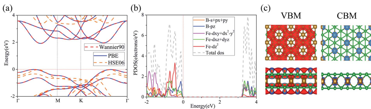
Fig. 3 The electronic properties of \text{FeB}_6 sandwich. (a) Electronic band structure of \text{FeB}_6 , the blue solid line represents the PBE band, the red dash line represents the Wannier interpolated band, the orange dash line represents the HSE06 band. (b) Total and partial densities of states (PDOS) of \text{FeB}_6 sandwich at HSE06 level. (c) Charge distribution of VBM and CBM for the \text{FeB}_6 sandwich at HSE06 level. The energy zero is set at the VBM for (a) and (b).
